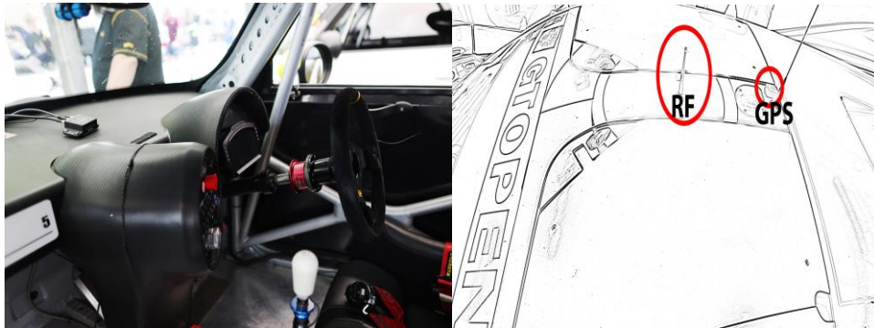
Installation examples, for the racelink, preferred position above the dashboard so that the driver can see the LEDs, for the antennas, RF and GPS outside in the roof.
